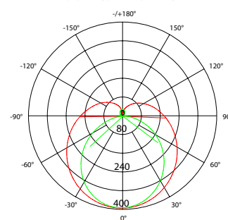
PHOTOMETRIC OF 1.2M LUMINAIRES
